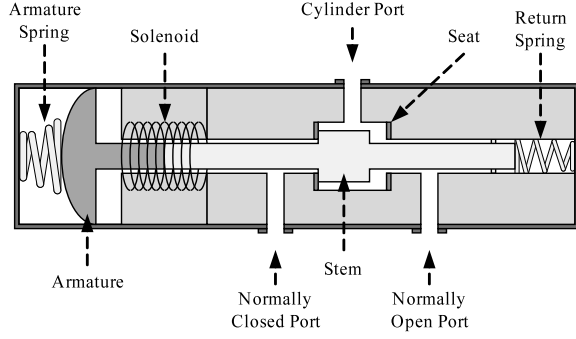
Figure 2: Three-way two-position solenoid valve.
