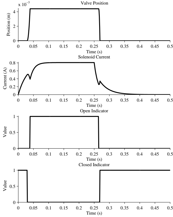
Figure 3: Nominal solenoid valve operation
