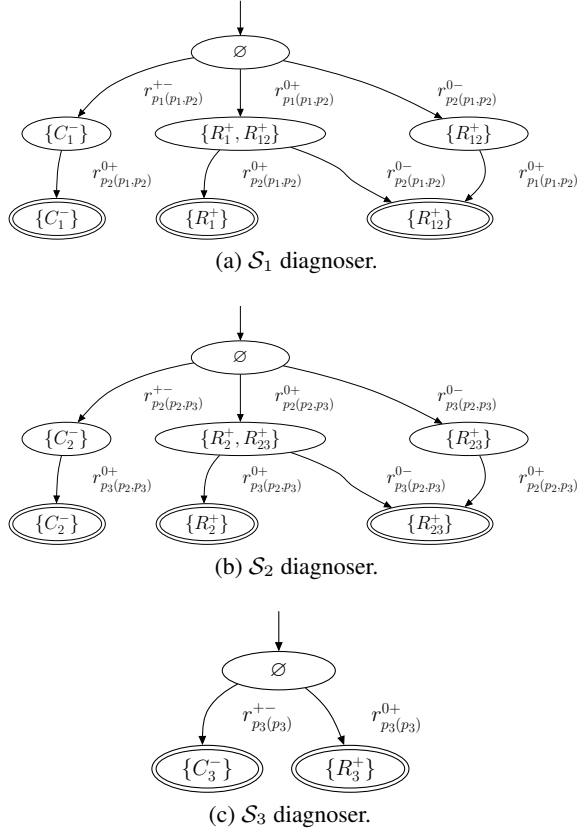
Figure 3: Local diagnosers for the three-tank system for F_1 = \{C_1^-, R_1^+, R_{12}^+\} , R_1 = \{r_{p_1(p_1,p_2)}, r_{p_2(p_1,p_2)}\} , F_2 = \{C_2^-, R_2^+, R_{23}^+\} , R_2 = \{r_{p_2(p_2,p_3)}, r_{p_3(p_2,p_3)}\} , F_3 = \{C_3^-, R_3^+\} and R_3 = \{r_{p_3(p_3)}\} .
