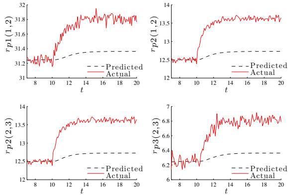
Figure 4: Three-tank predicted and observed flow outputs r_{p_1(p_1,p_2)} and r_{p_2(p_1,p_2)} for \mathcal{S}_1 , and r_{p_2(p_2,p_3)} and r_{p_3(p_2,p_3)} for \mathcal{S}_2 .
