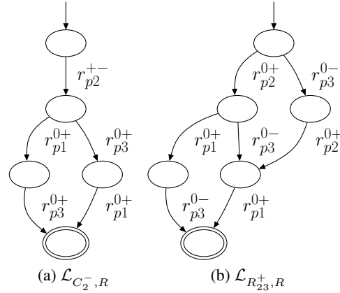
Figure 2: Fault models for some faults of the three-tank system, where R = \{r_{p_1}, r_{p_2}, r_{p_3}\} .
